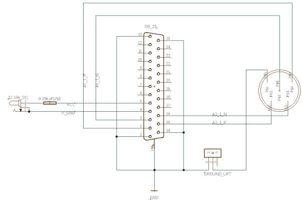
Wiring Diagram for TA5 model
